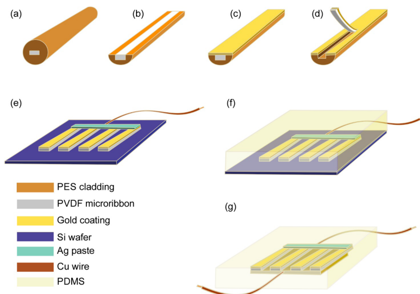
Figure 5. Fabrication process for the device produced using first step microribbons. (a) A 50 \mu\text{m} thick microribbon embedded single fiber is selected. (b) The fiber is longitudinally divided in two pieces. (c) The surface of the piece with the ribbon trapped is coated 50 nm gold. (d) After carving the PVDF microribbon out of the cladding, it is cut in equal pieces. (e) One side coated microribbons are aligned on a silicon substrate. Next, Ag paste and Cu wire electrodes are attached on the gold coated surface of the microribbons. (f) The structure is transferred onto a PDMS layer. (g) The back side of the PVDF microribbons are also coated with 50 nm gold, and the whole device is embedded in PDMS.
